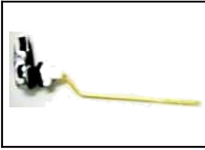
RR [ IMPORT ] RAM - 350 Side pull lever in brass rod in 45°c
