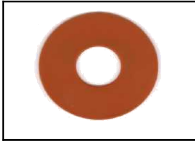
RR [ LOCAL ] RCY - K 200 H/D Flush valve silicon washer Out: 66mm x In: 24.5mm x T: 1.7mm
