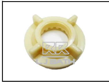
RR [ IMPORT ] RMC - P01 1/2" Plastic nut Dia: 43.7mm Thick: 12.8mm
