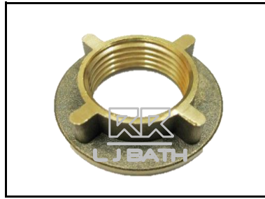
RR [ IMPORT ] RMC - B02 1/2" Brass nut Dia: 35mm Thick: 10.5mm
