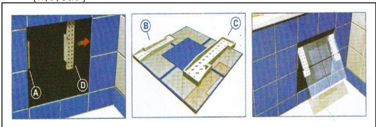
NICOLL [ IMPORT ] RAK-50 Access flap door's component hinges in ( 4 pieces ) [ A , B , C & D ]
