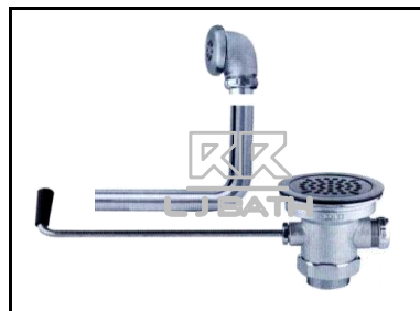
T & S [ USA ] RB - 3940-01 Twist waste 2"outlet c/w adaptor 2" to 1 1/2" & overflow assembly
