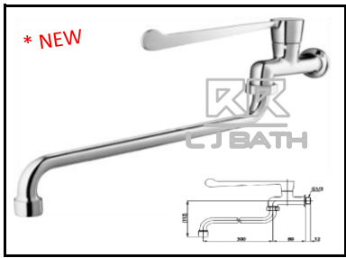
COTTO [ THAILAND ] CT1154C37 Lever tap c/w spout Lever: 200mm / Spout: 300mm
