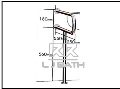
RR [ IMPORT ] BNH - 9010 U-Shape support rail 785 x 705 x 32
