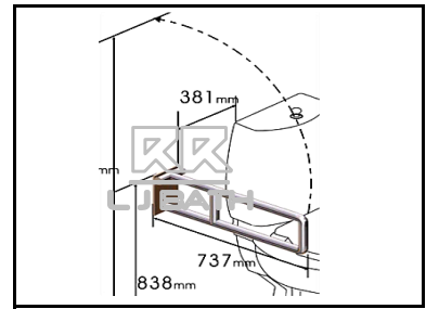
RR [ IMPORT ] BNH - 9032 Swing -up support rail 800 x 32
