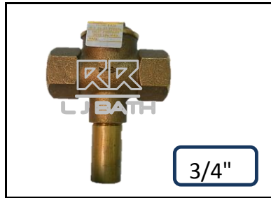
RMC [ Australia ] RMC- PS 75 Pressure Limiting Valve 3/4" Limit Pres 350 kPa[50.5 psi] 2000 kPa[290 psi]
