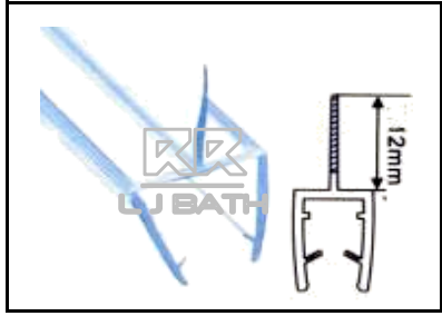
RL-P10 BR PVC SIDE & WIPE RAIL 10mm X 2.2m [ 86" ]
